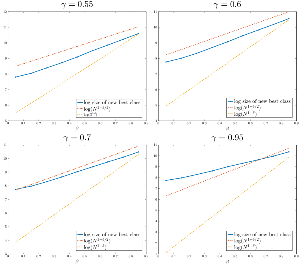
FIGURE 5. For N = 10^5 we compare the size of the “new best class” of the tournament ratchet immediately after a click (as observed by simulations) with \mathbf{a} = N^{1-\delta} and \mathbf{b} = N^{1-\delta/2} , which are the centers of attraction of the best and the second best class of the tournament ratchet (cf. Remark 3.6. b)). For various values of \gamma = \delta/(1 - \beta) , we consider (the logarithms of) these quantities as functions of \beta . Each data point was obtained by pooling the interclick times no. 5 to 30 from 20 simulations of the tournament ratchet for the corresponding parameter configuration. For a wide range of parameters with \gamma between 1/2 and 1, \mathbf{b} is a better fit for the size of the new best class than \mathbf{a} .
