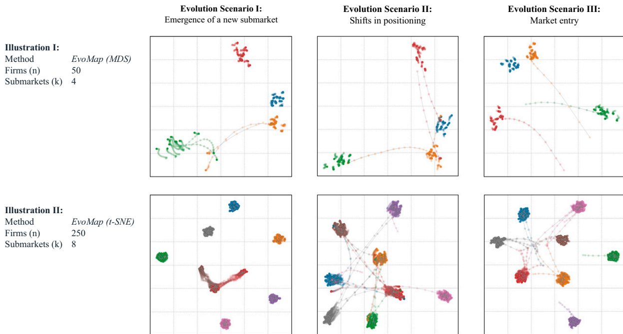
Figure 4. (Color online) Examples of Simulated Evolving Market Structures
