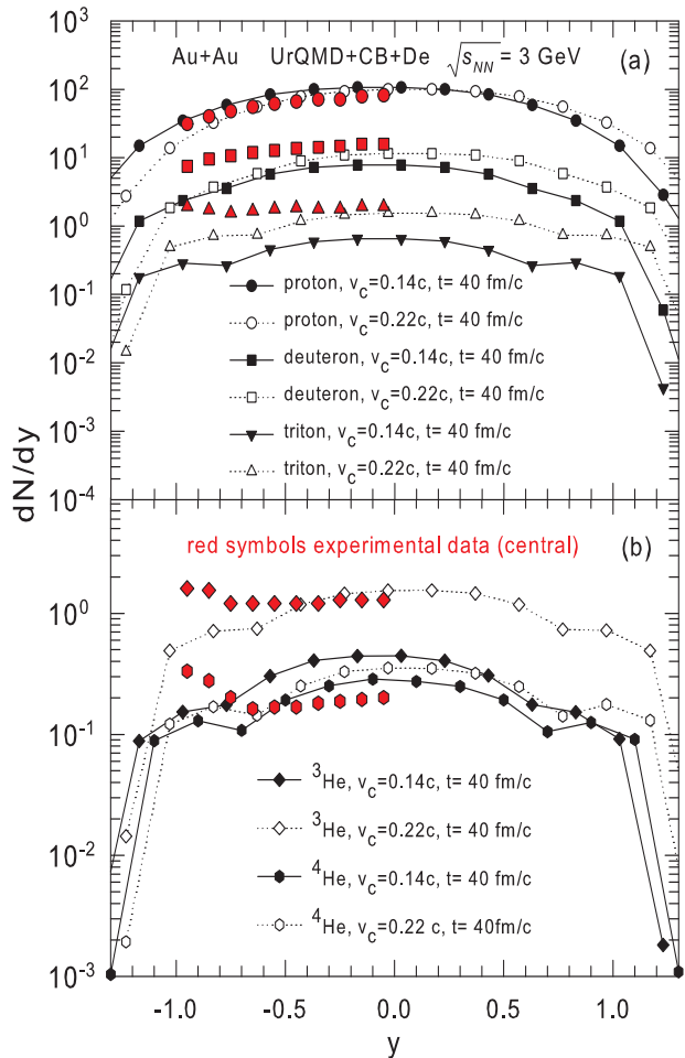
FIG. 5: (Color online.) Comparison of the calculations of the rapidity distributions of normal nuclei produced in central collisions with STAR experimental data [41]. Top panel (a) - protons, deuterons, tritons. Bottom panel (b) - {}^3\text{He} , {}^4\text{He} . The model parameters are indicated in the panels.
