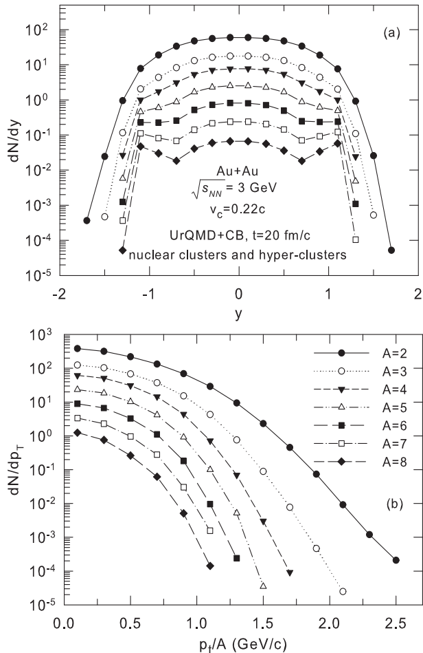
FIG. 3: Rapidity (top panel (a)) and transverse momentum per nucleon (bottom panel (b) overall rapidities) distributions of the excited baryon clusters, which have the mass numbers from A=2 to 8. Yields are per event.
