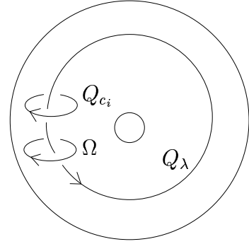
Figure 8.3: Decorated Hopf link in the annulus.
