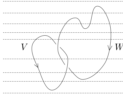
Figure 11.2: Decomposition of an oriented link diagram into simple pieces.
