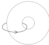
Figure 3.8: The additional arc for the closure.
