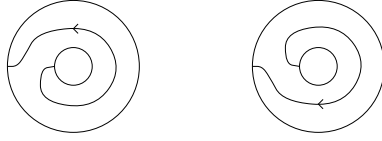
Figure 3.10: The arc a (at the left) and its inverse a^{-1} (at the right).
