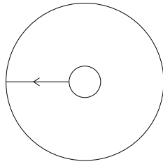
Figure 3.5: The identity e in C' .
