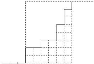
Figure 10.2: The dual Young diagram upside down.
