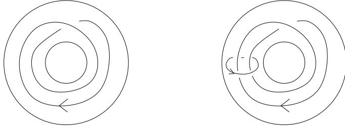
Figure 3.3: Encircling a diagram in the annulus.
