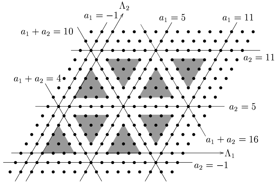
Figure 7.3: The lattice P(3) \subset V'(3) of elements a_1\Lambda_1 + a_2\Lambda_2 .
