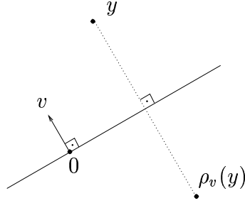
Figure 7.2: A point y and its mirror image \rho_v(y) .
