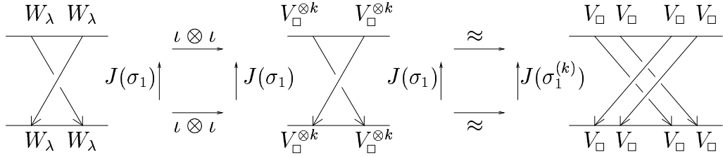
Figure 11.7: Homomorphisms arising at a crossing \sigma_1 in the braid \beta and the corresponding multiple crossings \sigma_1^{(k)} in the braid \beta^{(k)} shown in the case k = 2 .
