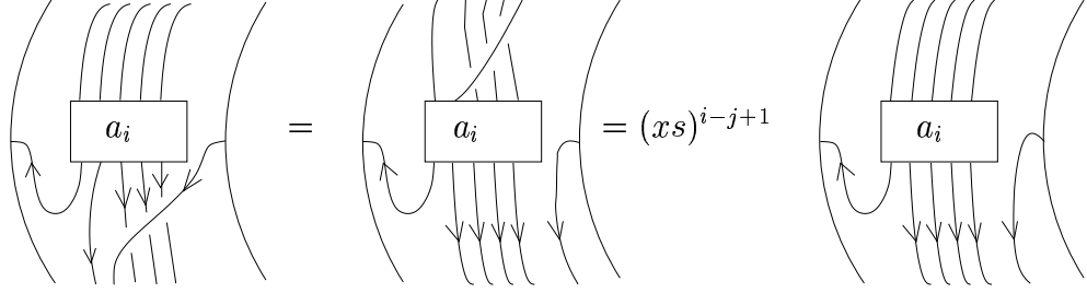
Figure 3.12: Moving crossings around in the annulus.
