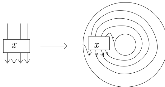
Figure 3.9: Map \Delta' from H_n to C' .
