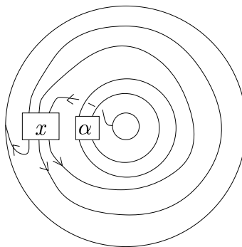
Figure 3.7: Operation of C on C' from the left.
