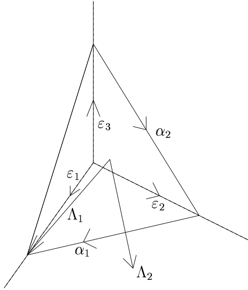
Figure 7.1: The vector space V(3) .
