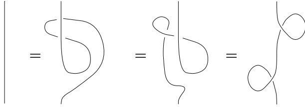
Figure 2.6: The Whitney-trick realizes a cancellation of curls via a regular isotopy.
