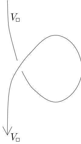
Figure 11.3: A positive curl.
