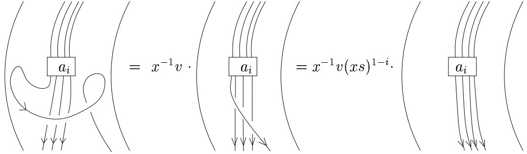
Figure 3.13: The closure of A'_i a .
