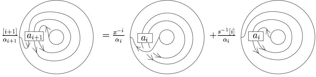
Figure 3.11: Depiction of lemma 3.4.1.
