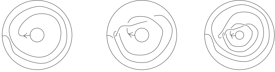
Figure 3.4: The multiplication in C' .
