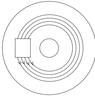
Figure 3.2: The closure map from H_n to C .
