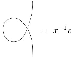
Figure 2.7: A derived relation in \mathcal{S}(\mathcal{F}, \Gamma) .
