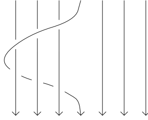
Figure 2.10: The n -string braid T(j) for n = 7 and j = 4 .
