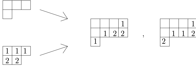
Figure 1.1: The two extensions of (3, 1) by (3, 2) to (4, 4, 1) .
