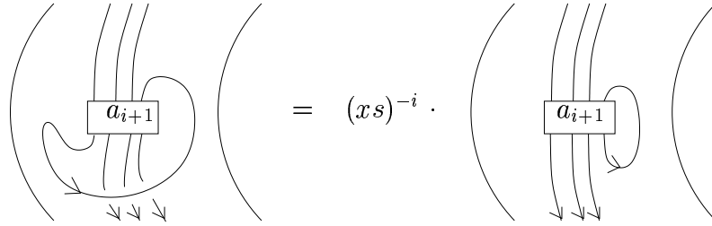
Figure 3.14: The closure of A'_i .
