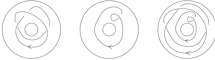
Figure 3.1: The multiplication in the skein of the annulus C .
