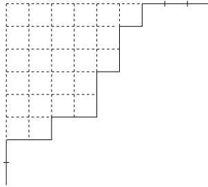
Figure 10.1: Young diagram \lambda = (6, 5, 5, 4, 4, 2) with extended lines in the case N = 8 and l = 9 .
