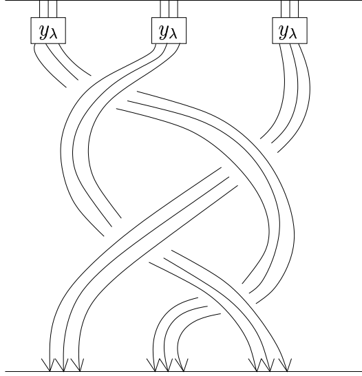
Figure 11.5: The element y_\lambda^{\otimes d} \beta^{(k)} of H_{kd} in the case \beta = \sigma_1 \sigma_2^{-1} \sigma_1 \sigma_2^{-1} corresponding to the figure-eight knot with zero-framing, with |\lambda| = k = 3 and d = 3 .
