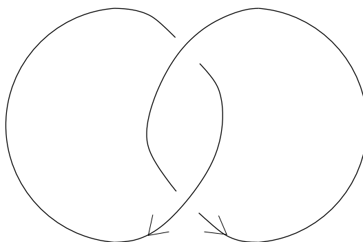
Figure 4.1: The Hopf link.
