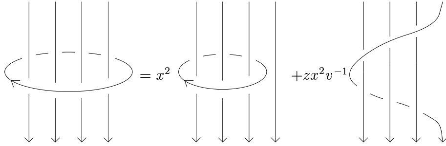
Figure 2.12: An equivalent depiction of the equation in figure 2.11.
