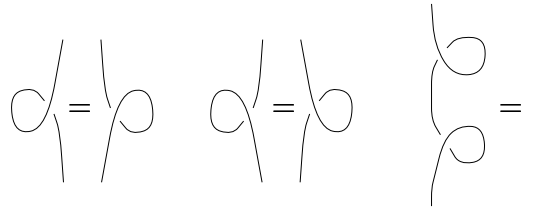
Figure 2.8: Moves in order to handle curls in diagrams.
