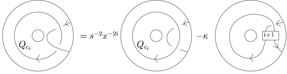
Figure 5.1: Pulling a string through Q_{c_i} .
