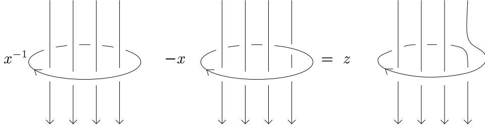
Figure 2.11: A relation in the Hecke algebra H_n .
