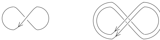
Figure 4.2: The unknot with framing 1 and its 2-parallel.
