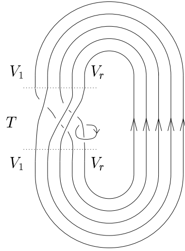
Figure 11.4: The \mathcal{A} -invariant of \hat{T} can be computed as the trace of \mu J(T) .
