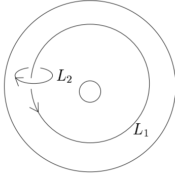
Figure 8.2: The Hopf link L_1 \cup L_2 in the annulus.
