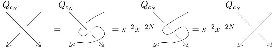
Figure 5.2: Pulling an oriented arc through a component decorated with Q_{c_n} .
