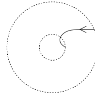
Figure 3.6: A map between different skeins of the annulus after turning the annulus over.
