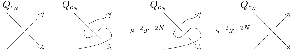
Figure 5.3: Pulling a differently oriented arc through a component decorated with Q_{c_n} .
