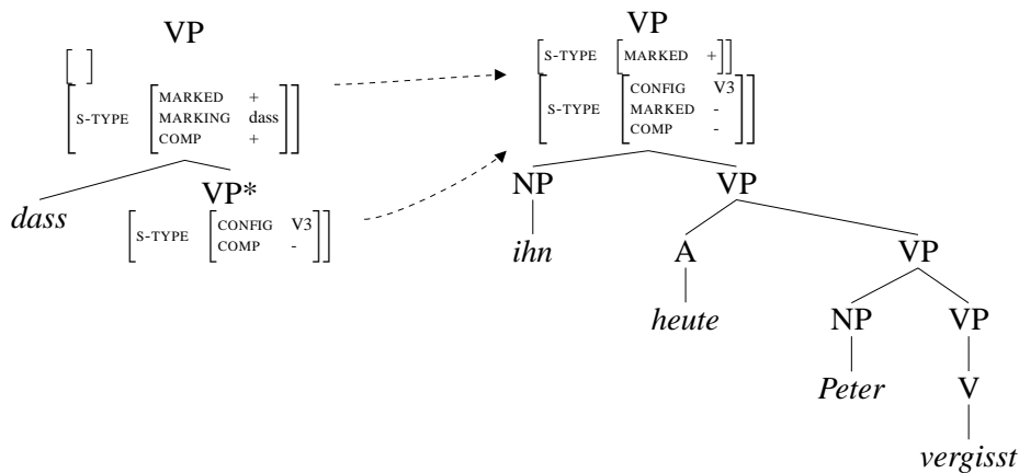
Figure 7: Complementizers
