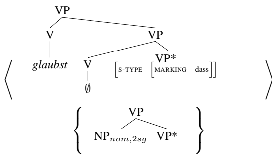
Figure 8: Bridge verbs
