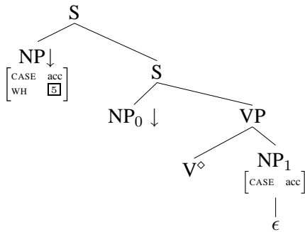
Figure 9: Feature reduced XTAG tree for object extraction (Fig. 15.1 therein)
