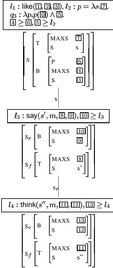
Figure 7: Abriged derivation tree and semantics for (19)
