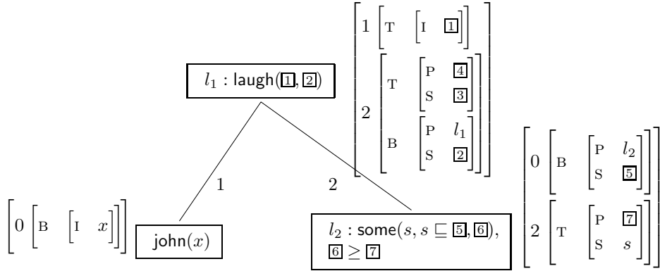
Figure 2: Semantic representations for (9)
