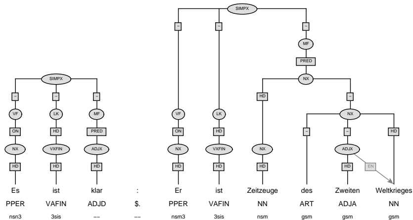
Figure 3: A tree containing a phrase internal named entity.
