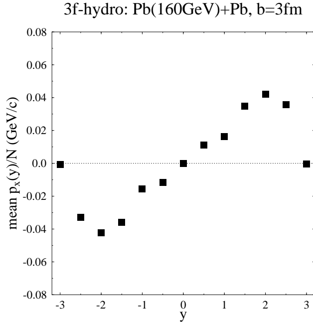
Figure 3: Directed nucleon flow \langle p_x^{dir}/N \rangle(y) in Pb+Pb -collisions ( b = 3 \text{ fm} ) at CERN-SPS.
