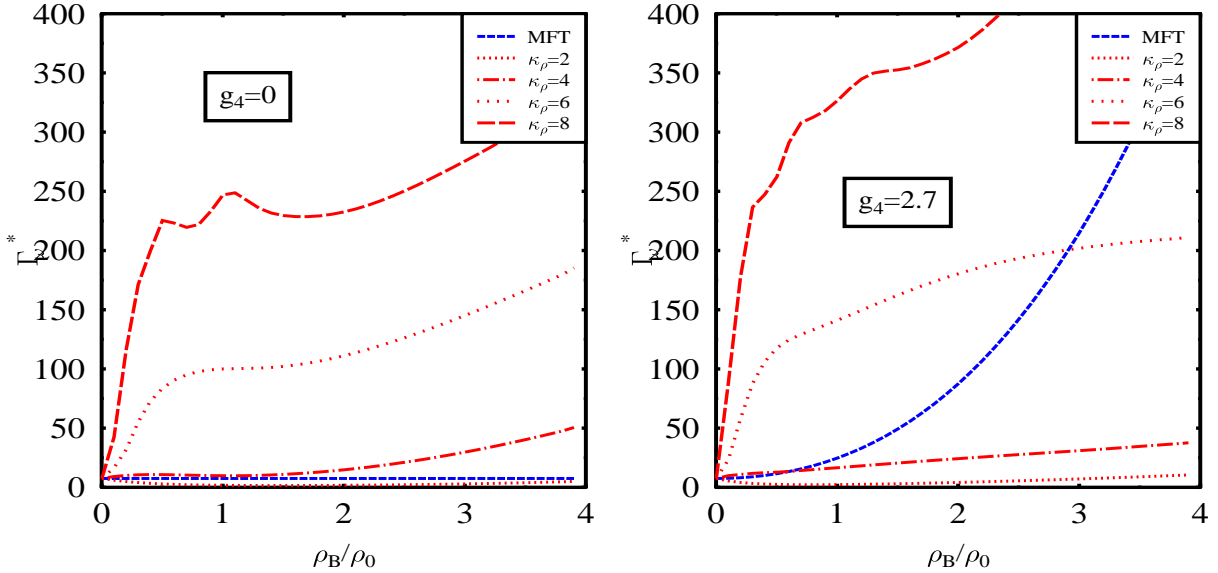
FIG. 10: Decay width of \omega meson in the absence and presence of the Dirac sea effect. For the channel \omega \rightarrow \rho\pi , the \rho meson properties are determined with the nucleon-rho vector coupling, g_{N\rho} , as from the chiral model, which is compatible with the symmetry energy and, the tensor coupling, \kappa_\rho is taken as a parameter.
