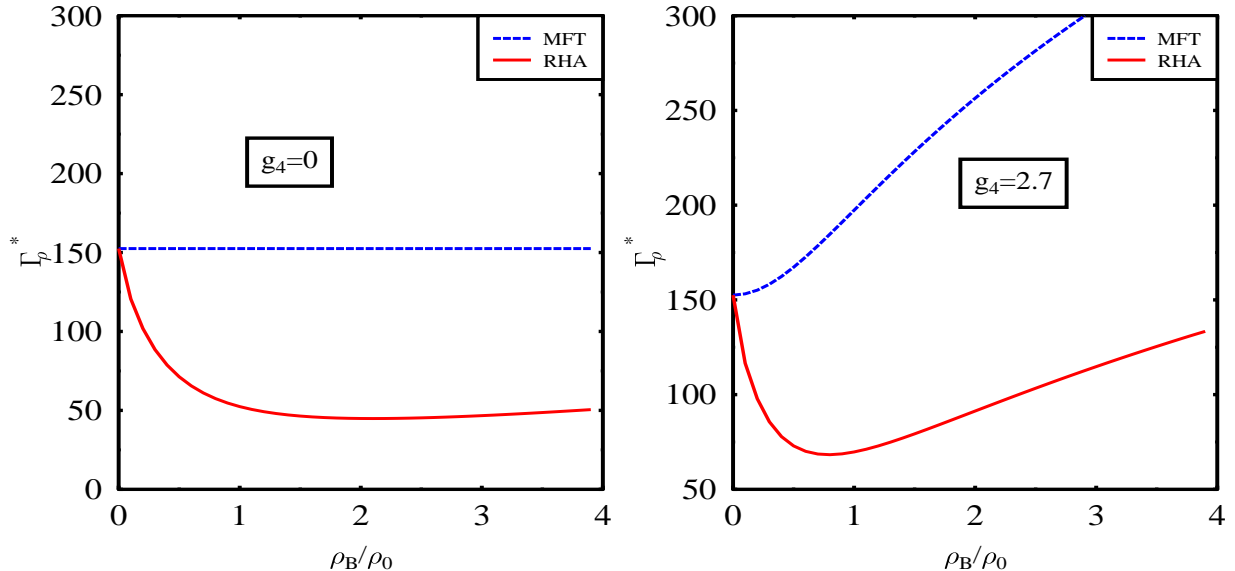
FIG. 6: Decay width of \rho meson in the absence and presence of the Dirac sea effect with the couplings fitted from the NN scattering data.
