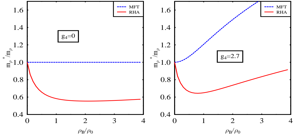
FIG. 5: Effective \rho meson mass without and with the Hartree contributions, with the nucleon-rho vector and tensor couplings, as fitted from the NN scattering data ( g_{N\rho}=2.63 , \kappa_\rho = 6.1 ). The Hartree approximation gives rise to the decrease of the \rho mass in the medium.
