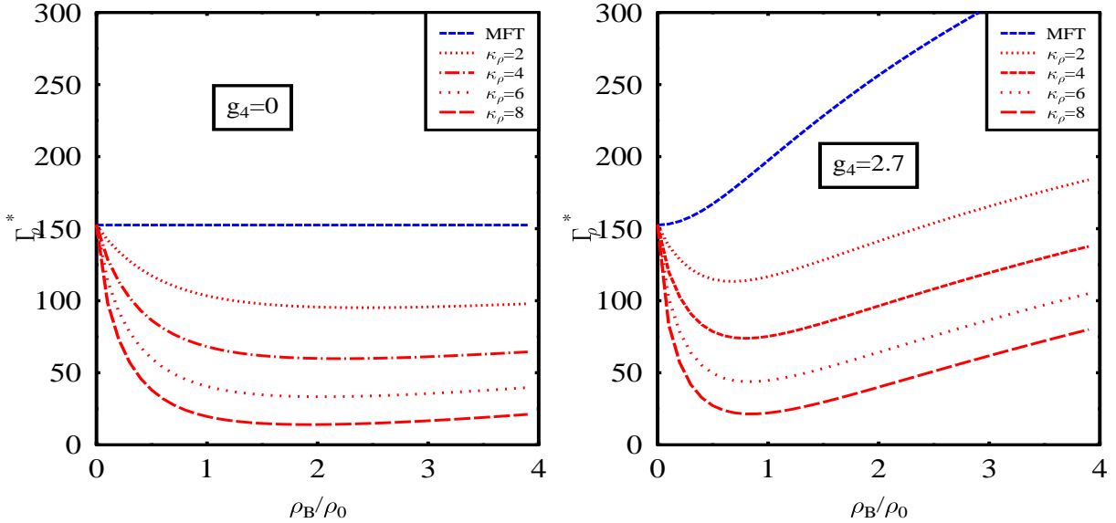
FIG. 8: Decay width of \rho meson in the absence and presence of the Dirac sea effect with the nucleon-rho vector coupling, g_{\rho N} , as from the chiral model, which is compatible with the symmetry energy. The tensor coupling, \kappa_{\rho} is taken as a parameter.
