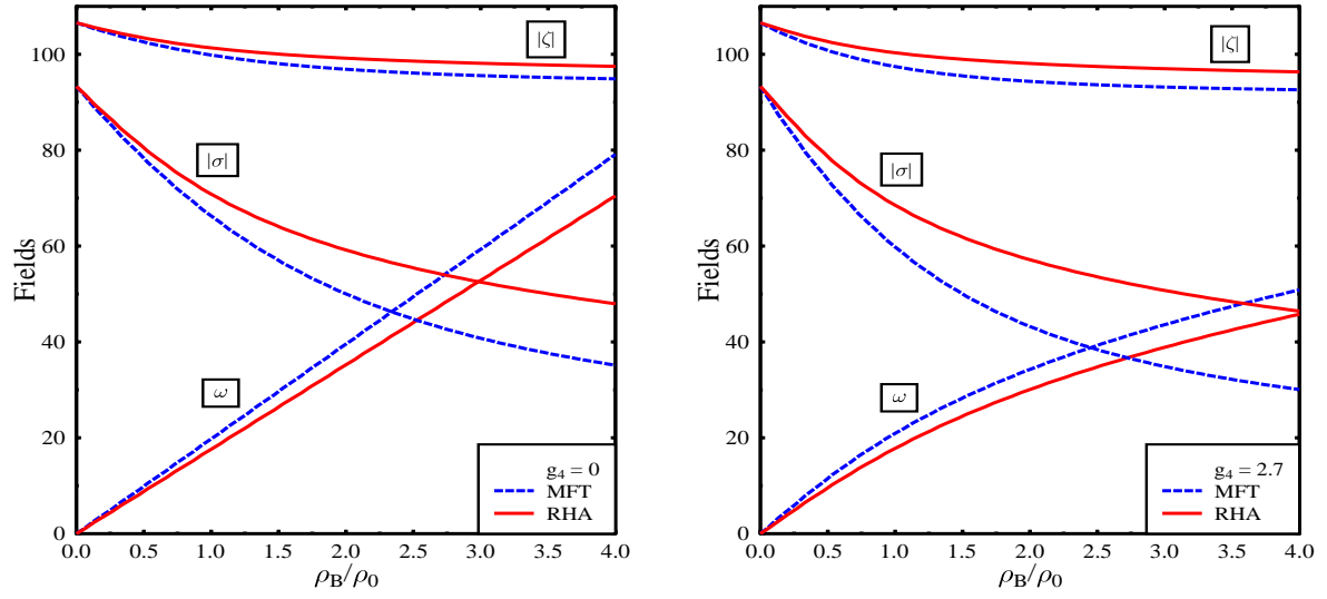
FIG. 2: Scalar fields \sigma , \zeta and vector field \omega as a function of density in the Mean-Field and in the Hartree-Approximation.
