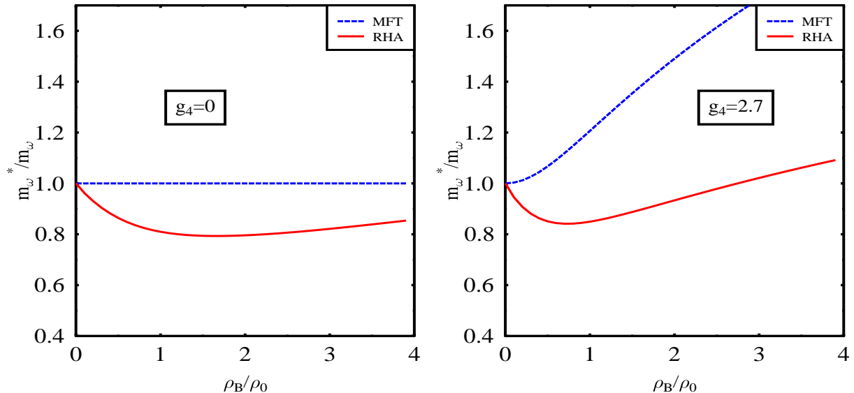
FIG. 4: Effective \omega meson mass in the mean field approximation and including the Hartree contributions. Left: no quartic vector-meson interaction. Right: Including \omega^4 interaction. There is significant drop of the vector meson mass due to the Dirac sea effect, which is not seen in the mean field approximation.
