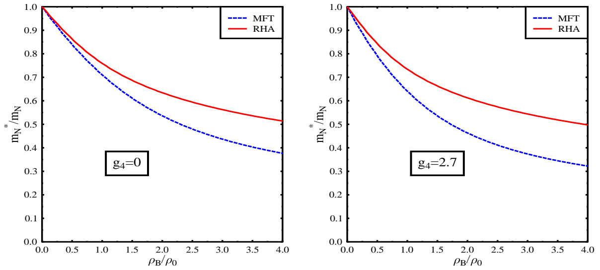
FIG. 3: Effective nucleon mass as a function of density in the Mean-Field and in the Hartree-Approximation.
