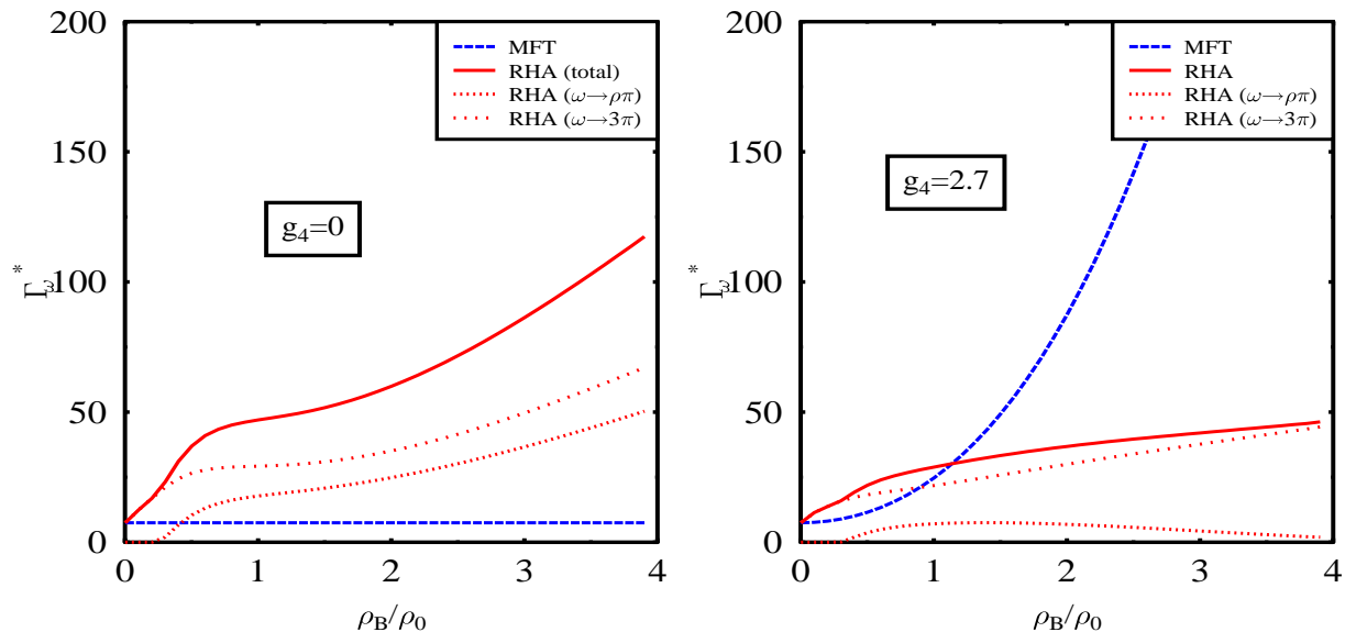
FIG. 9: Effective decay width of \omega meson without and with the Hartree contributions. The decay width has contributions from \omega \rightarrow 3\pi as well as \omega \rightarrow \rho\pi . The latter becomes accessible due to stronger medium modification of the \rho meson mass as compared to the \omega mass. The MFT has no contribution from the process \omega \rightarrow \rho\pi .
