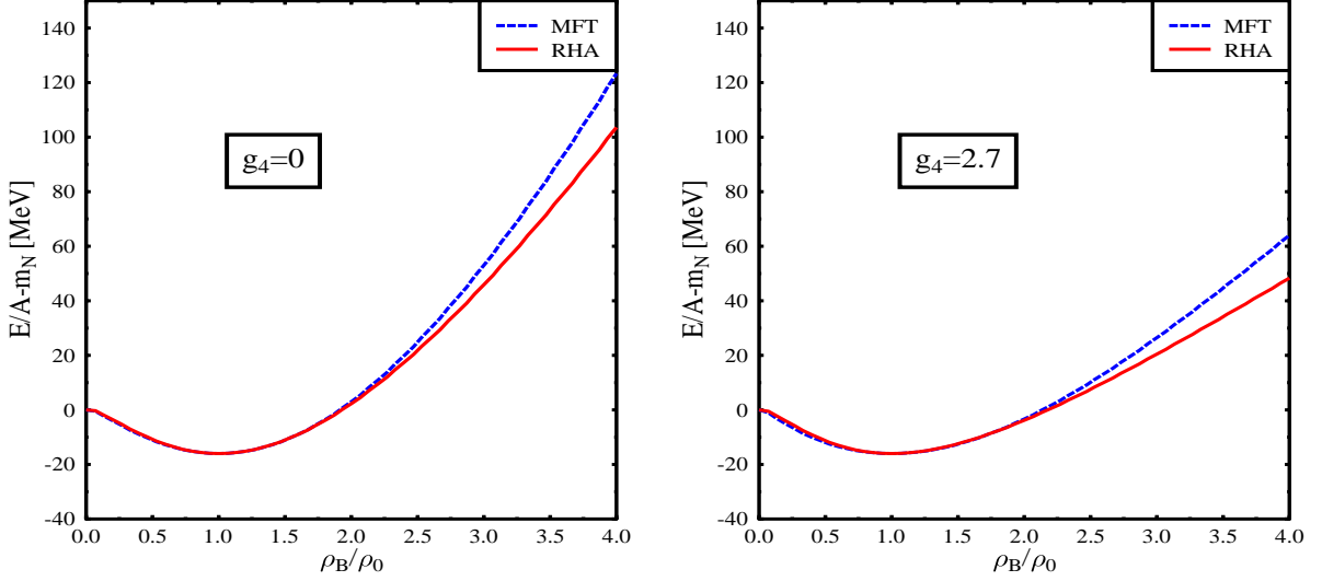
FIG. 1: Binding energy per particle as a function of density in the Mean-Field and in the Hartree-Approximation.
