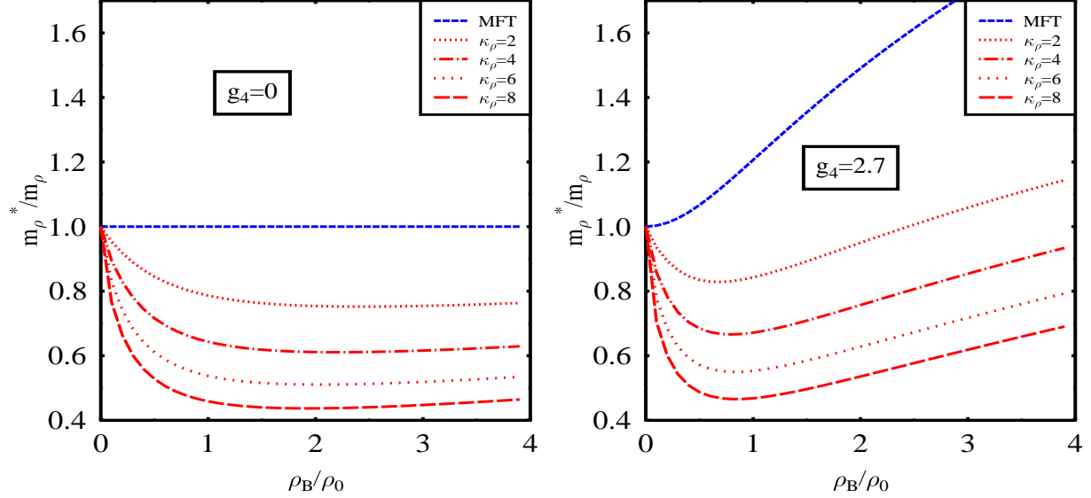
FIG. 7: Effective \rho meson mass without and with the Hartree contributions, with the nucleon-rho vector coupling, g_{N\rho} , as from the chiral model, which is compatible with the symmetry energy. Since we do not know the medium dependent tensor coupling, \kappa_\rho , it is taken as a parameter. The Hartree approximation gives rise to the decrease of the \rho mass in the medium, which is seen to be quite sensitive to the nucleon- rho tensor coupling.
