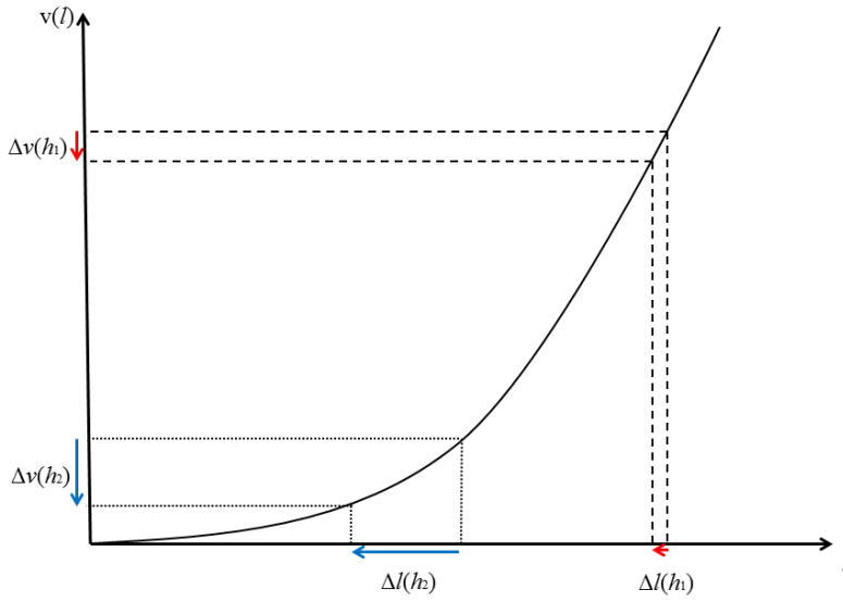
Figure 2: Example for \partial^2 v(\hat{y}, \theta, h) / (\partial \theta \partial h) < 0 .
