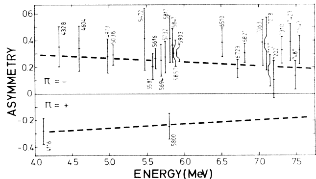
FIG. 2. Combined asymmetries from the ^{206}\text{Pb}(\gamma_{\text{pol}}, \gamma) measurements with linearly polarized bremsstrahlung of 10 and 12 MeV end-point energy.
