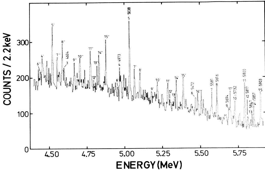
FIG. 1. Part of a ^{206}\text{Pb}(\gamma, \gamma) spectrum measured with 7-MeV bremsstrahlung at a scattering angle of 127^\circ .
