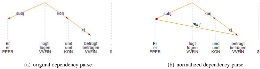
Figure 2: Illustration of normalizing dependency parses with verb coordination.
