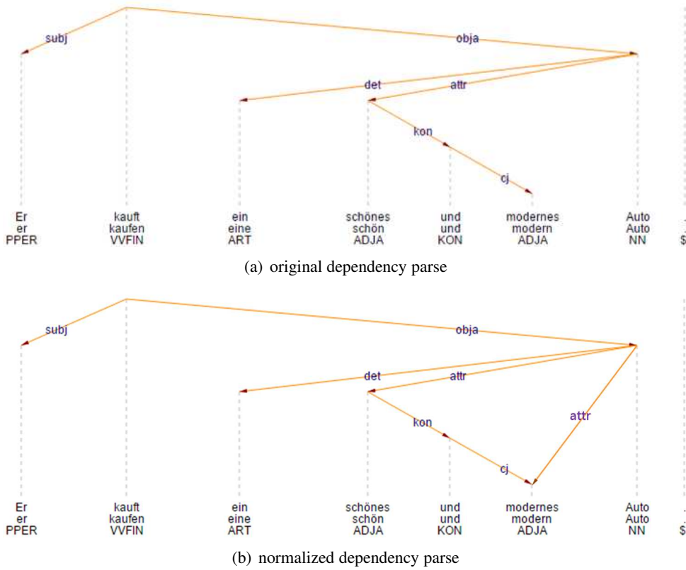
Figure 3: Illustration of normalizing dependency parses with adjective coordination.
