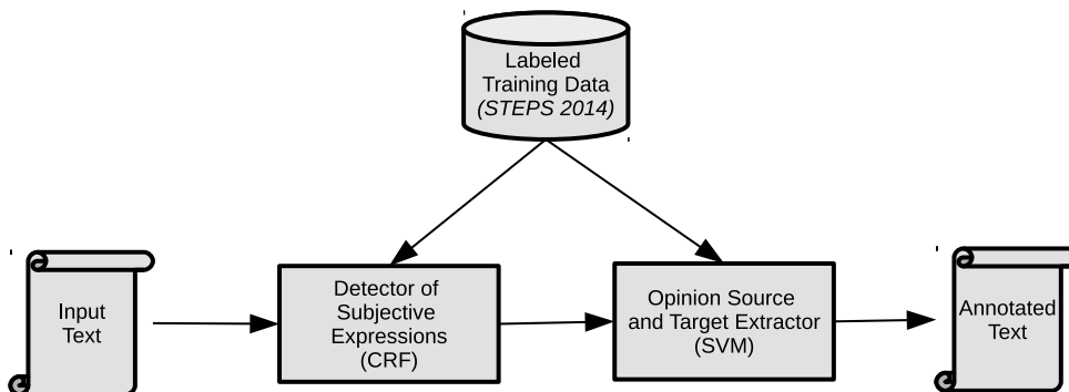
Figure 4: Processing pipeline of the supervised system.
