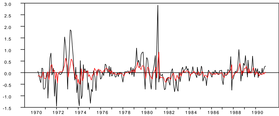
Figure 5: Contribution of the Markov chain to short rate changes RSH-VAR(1) model for differenced short rate and spread
