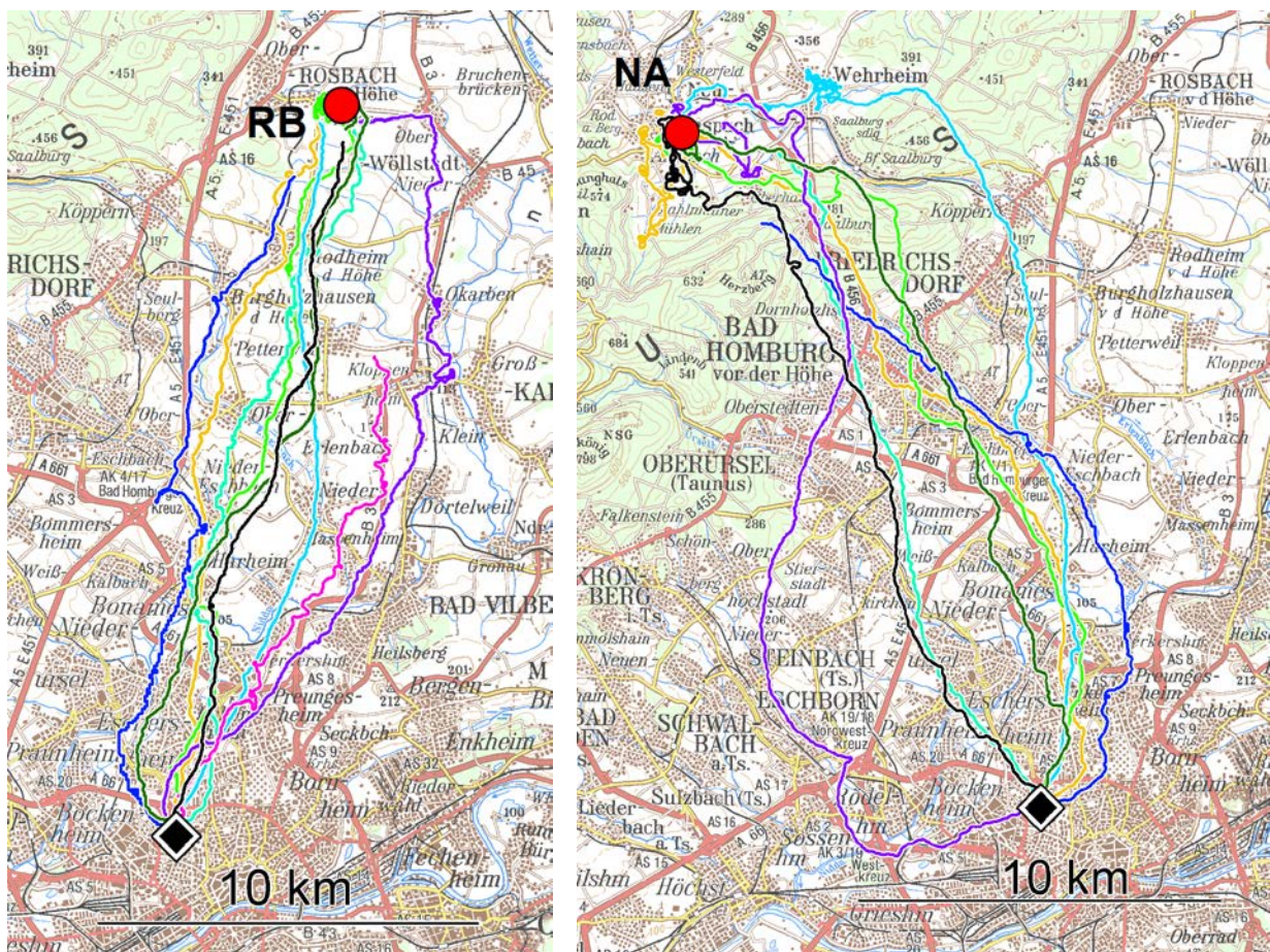
Fig.S2. Tracks recorded in 2010 (see also Fig. 2 in the main text). Red dots, release sites; black diamond, loft at Frankfurt am Main. The tracks of individual birds are given in different color, see legend.- From RB, 19.2 km from the loft, all birds flew singly; from NA, 21.3 km from the loft, birds 08-797 and 08-755 flew together.
