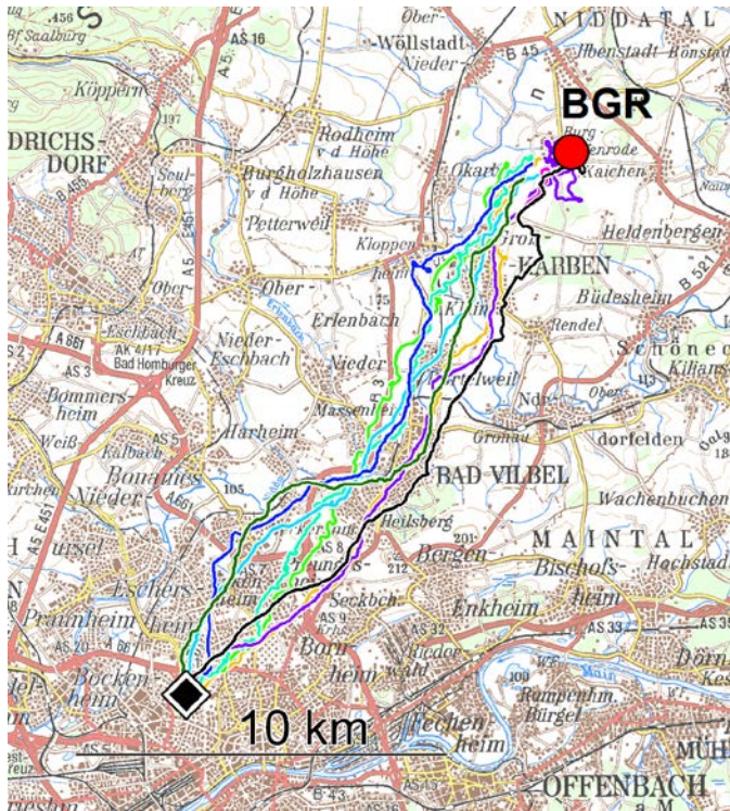
Fig.S2. Tracks recorded in 2010. Red dots, release sites; black diamond, loft at Frankfurt am Main. The tracks of individual birds are given in different color, see legend.- From BGR, 17.3. km, 08-755 and 08-797 flew together.
