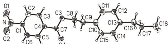
Fig. 1. Solid state structure of 8 .
