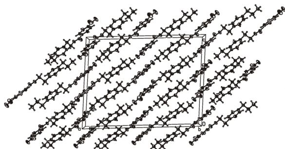
Fig. 2. Unit cell of 8 .
