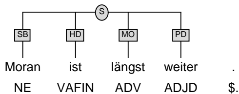
Figure 5: Negra annotation without unary nodes.
